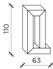
FRONTE | FRONT
