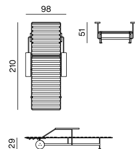
SUNLOUNGER + ARMRESTS dimensions 98 × 210 × 51 cm
