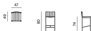
BASRSTOOL dimensions 47 × 49 × 80 cm
